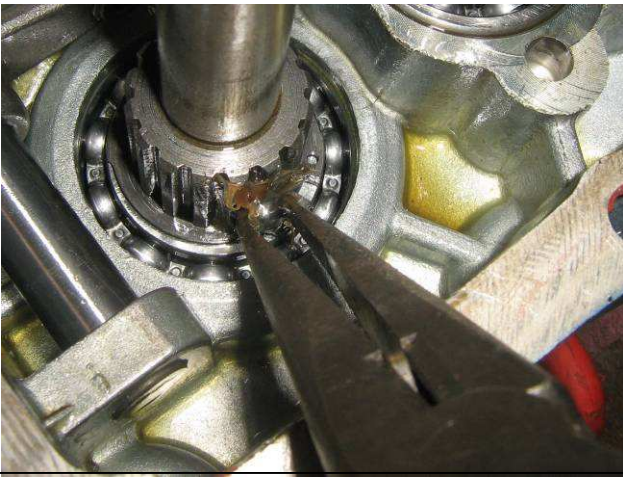
23. STICK THE BALLS INTO THE GREASE BLOBS ON EITHER END OF SPRING HOLE. (HOLE IN THE PLOT: THE INTERNAL PTO SHIFT LEVER IS STILL IN PLACE IN A FEW OF THESE PICS...BAD PHOTO SEQUENCING ON OUR PART, PLEASE IGNORE. RE-ASSEMBLY IS EASIER WITH LEVER OUT OF HOUSING.)
